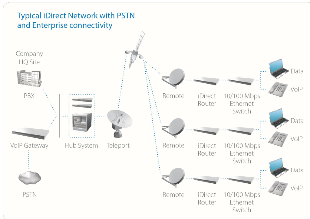
Figure 1: iDirect VoIP Solution
