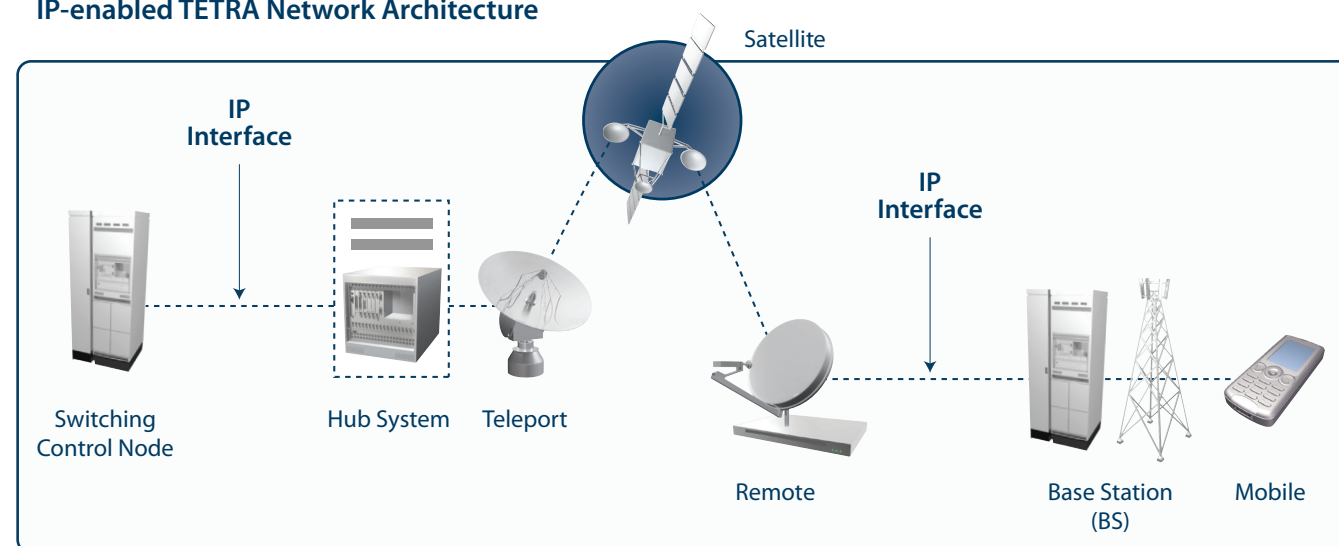
A TETRA Base Station at a remote site connects via an iDirect remote satellite router to an iDirect hub that is co-located with a TETRA Switching Control Node.
