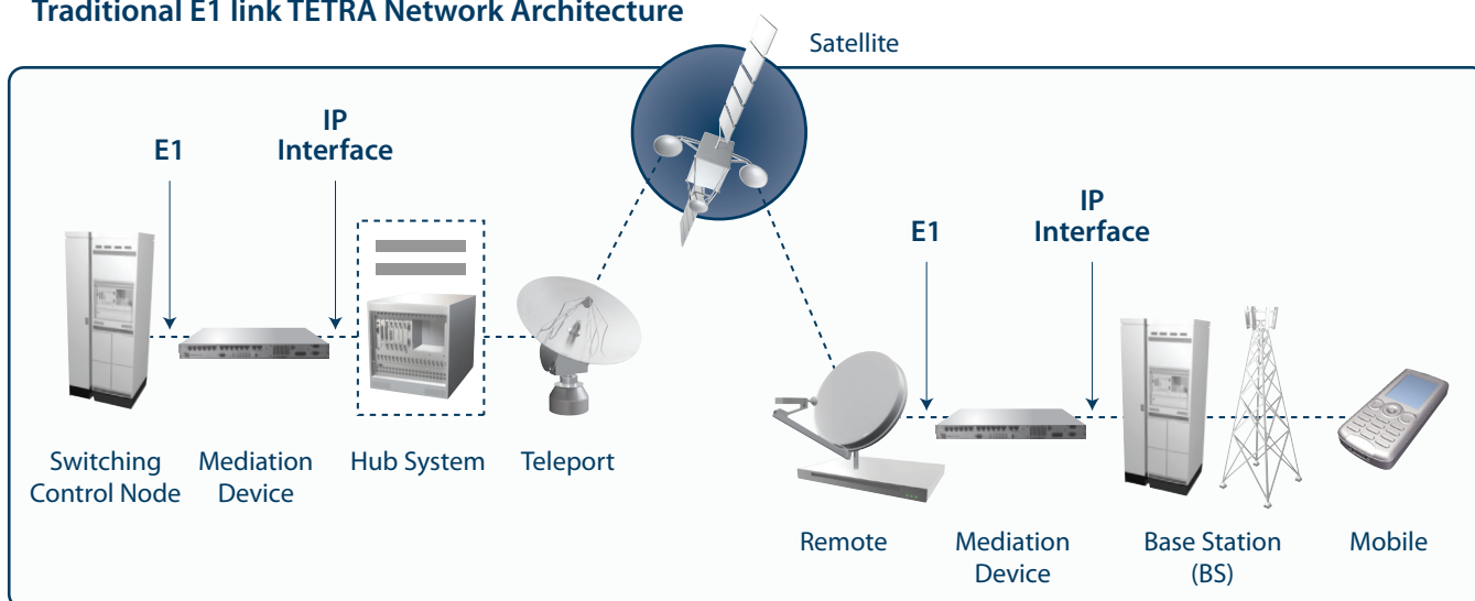
A TETRA network using E1 links connects via mediation devices at the hub and remote locations to an iDirect satellite network IP link.
