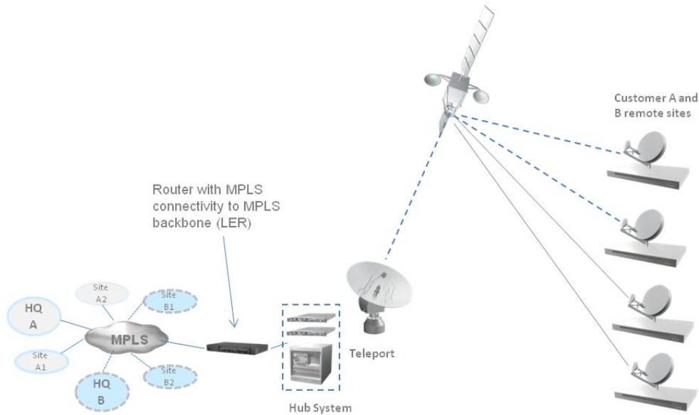
Figure 1: Integrate Customer Sites to MPLS Backbone
